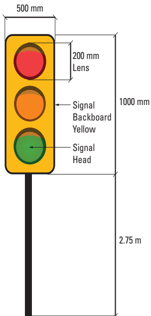
Figure 4.9 Portable Lane Control Signal
